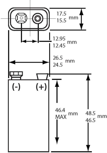
Dimensions shown are IEC standards
