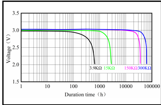
4. Capacity VS. Load Resistance
