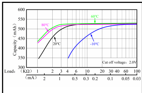
4. Capacity VS. Load Resistance
